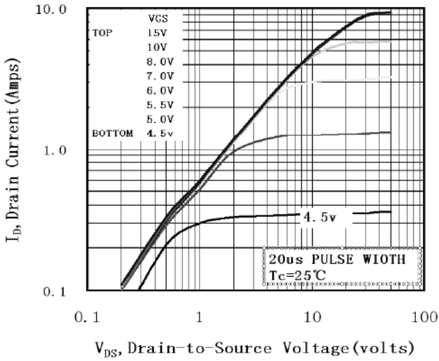
Output Characteristic
