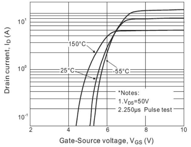
Transfer Characteristic
