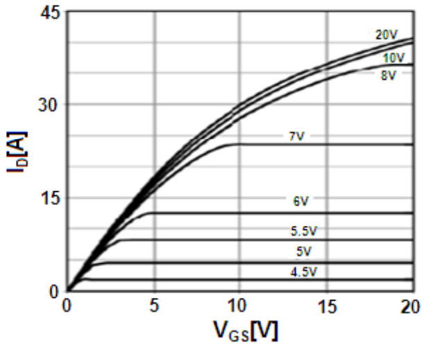
Output Characteristic
